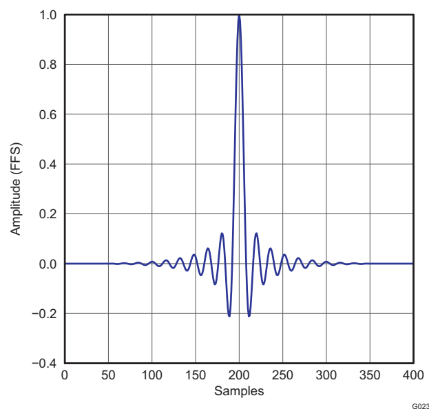
Figure 17. Normal ×8 Interpolation-Filter Impulse Response
