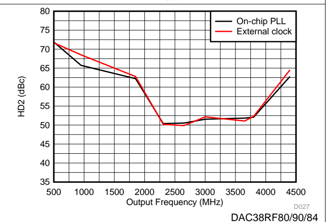
Figure 12. HD2 vs Output Frequency Over Clocking Option
